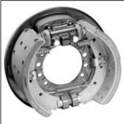
Front and rear axle: Simplex Expanding Wedge Drum Brake 410 × 200 ZE
